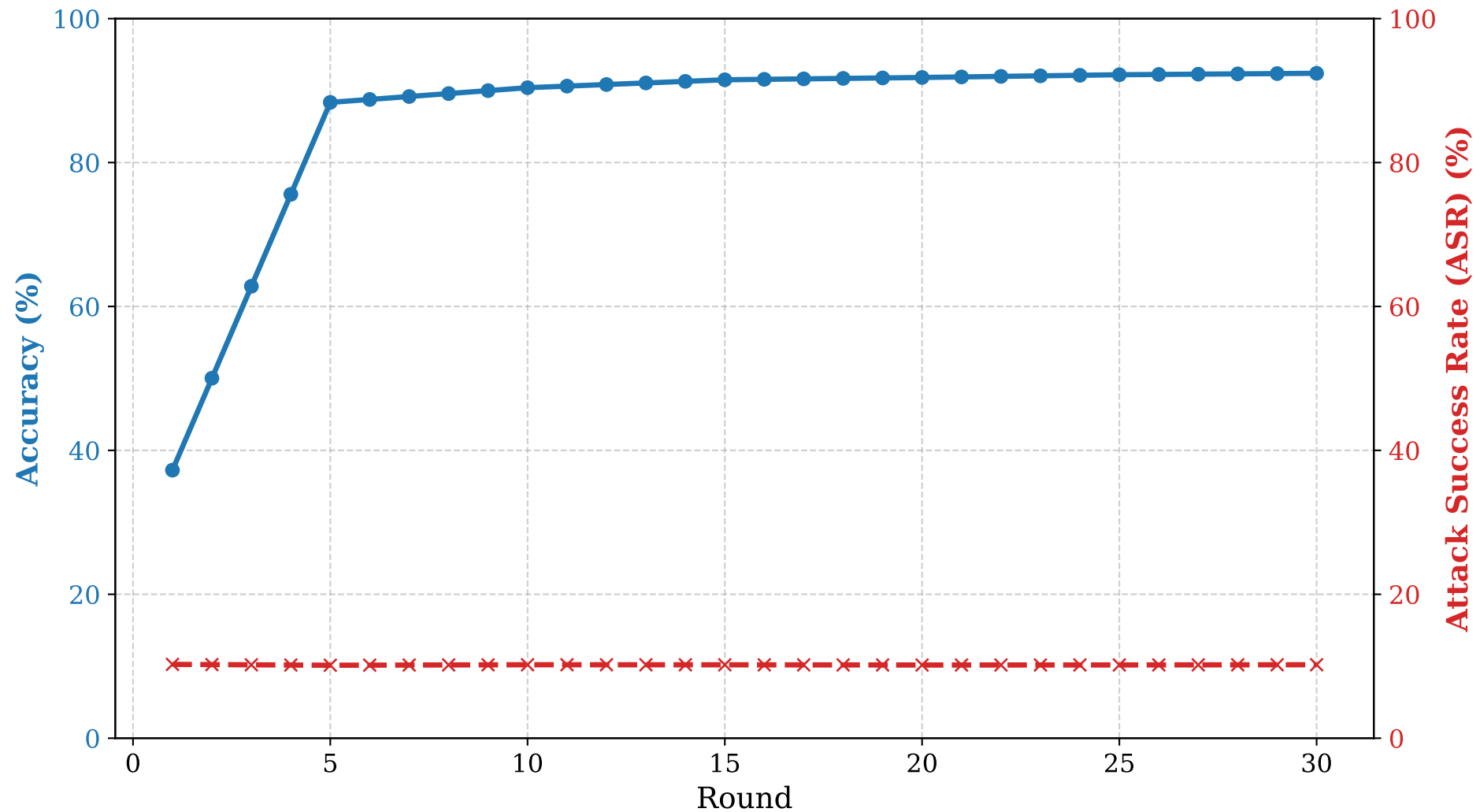
Convergence & Backdoor Suppression across 30 Rounds
